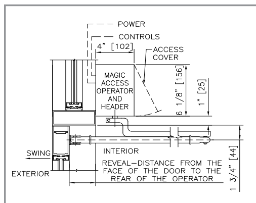
SURFACE MOUNTED VISIBLE "OUT"
