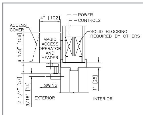
SURFACE MOUNTED VISIBLE "IN"
